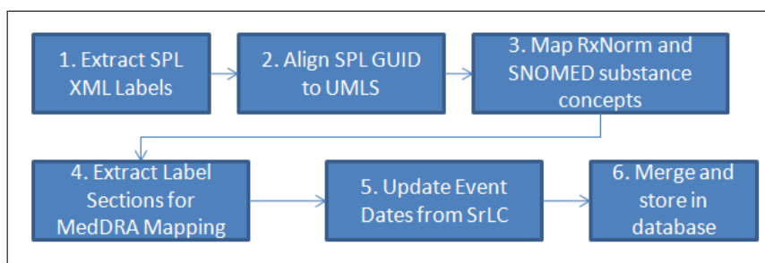
Fig. 1 PVLens Processing Pipeline Overview. [GUID = Global Unique Identifier, SrLC = Safety-Related Label Change]
